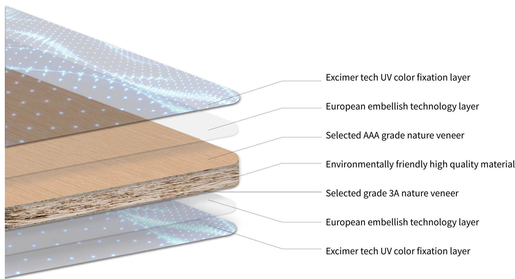
Nature veneer board structure layer
